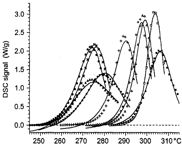
Fig. 1 Thermal decomposition of cellulose in hermetically sealed sample holders [1]. Nine high pressure DSC experiments are shown, differing from each other by the sample mass and/or the amount of water placed into the sealed sample holders. The experiments are represented by different symbols. The solid lines stand for the simulated curves which were obtained by a simultaneous least squares evaluation based on reaction scheme (4)
