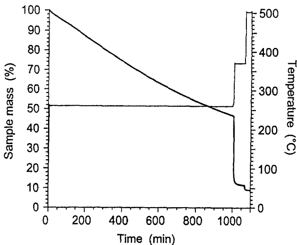
Fig. 2 Thermal decomposition of cellulose in open sample pans. A typical thermogravimetric experiment is shown which were used by the authors to check the validity of reaction schemes (5), (6) and (8). Here the bold and thin lines represent the experimental sample mass and temperature curves, respectively
