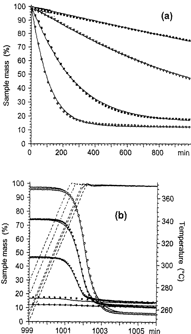
Fig. 3 Simultaneous least squares evaluation of five cellulose TG curves during a long isothermal section (a), and during the subsequent heating to a second, high temperature isothermal section (b), respectively [2]. The evaluation was based on reaction scheme (8). The symbols ( \circ \bullet \nabla \blacksquare \diamond ) and the solid lines represent the observations and the simulated curves, respectively. The following low temperature isothermal sections were employed: 120 min at 250°C ( \circ ), 999 min at 250°C ( \bullet ), 999 min at 260°C ( \nabla ), 999 min at 275°C ( \blacksquare ) and 999 min at 286°C ( \diamond ), respectively. In (b) the dashed lines represent the temperature and the time scale of the experiment with 120 min preheating ( \circ ) starts at 120 min
